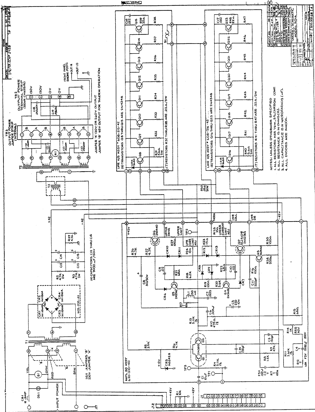
Figure 7-2. Model 501A Overall Schematic, Dwg. No. 505-002-6X
