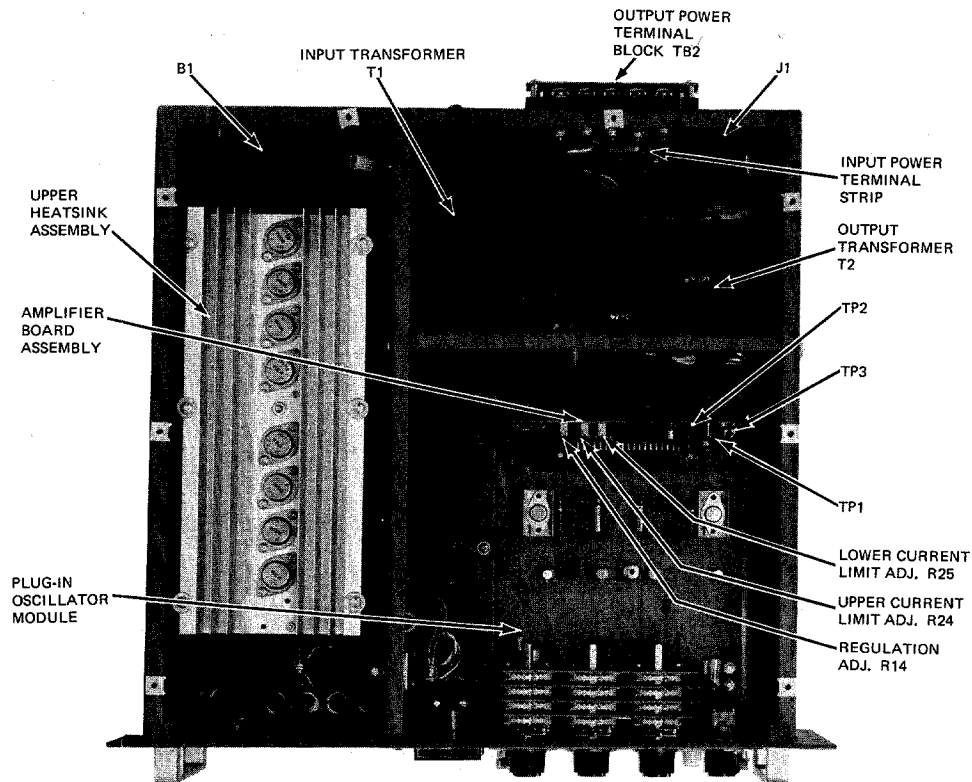
Figure 5-1. Model 501A Top View
