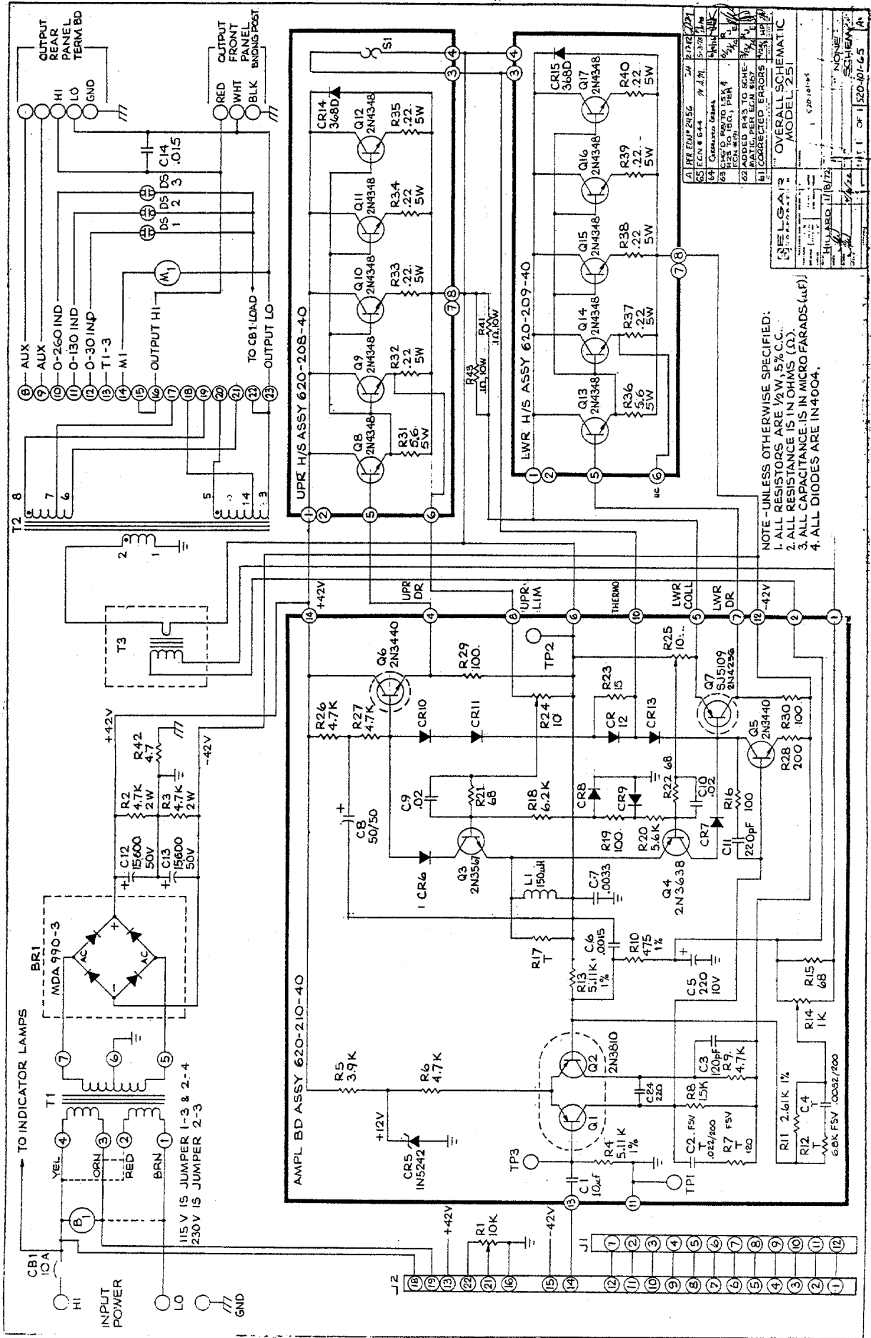
Figure 7-1. Model 251 Overall Schematic, Dwg. No. 520-101-6X
