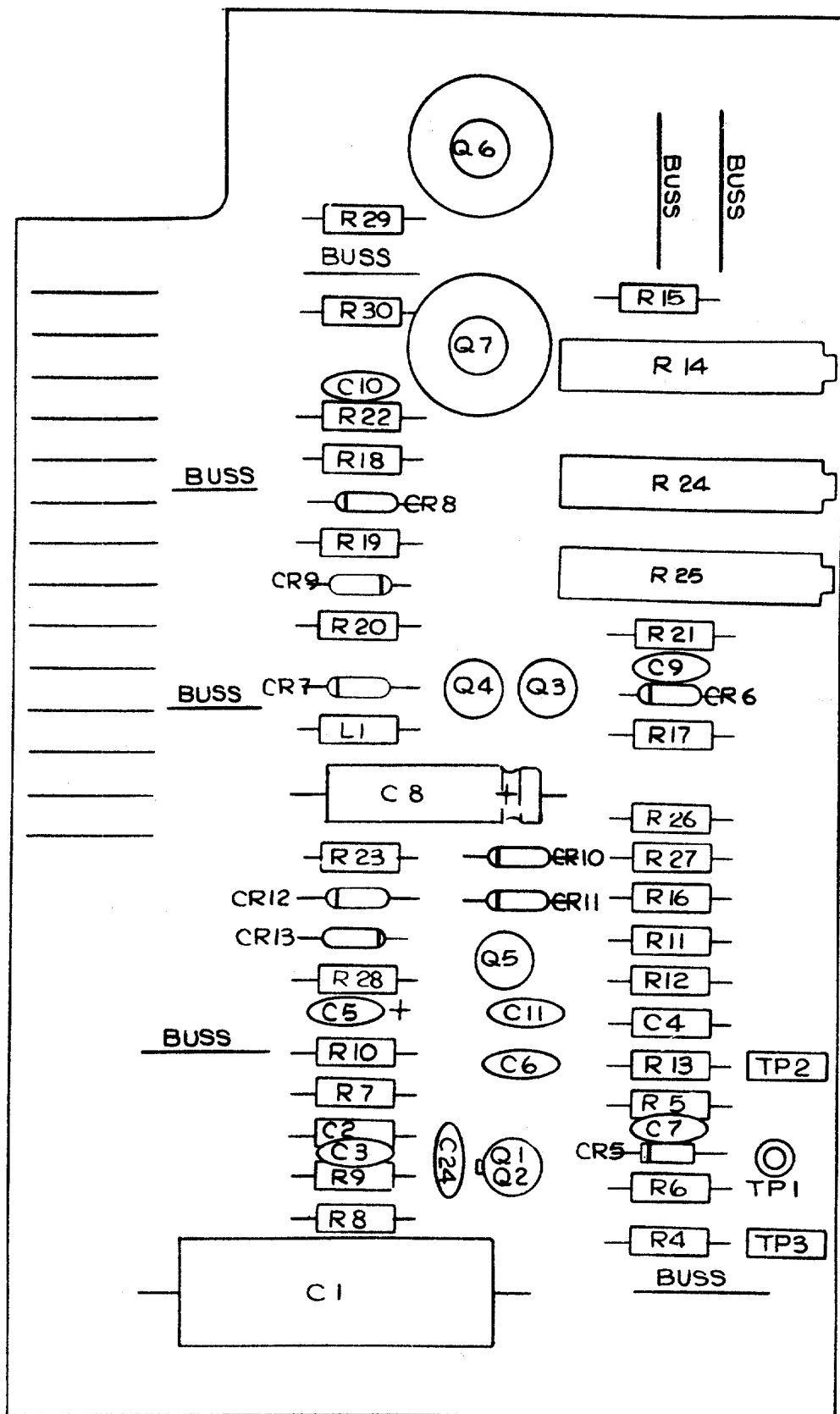
Figure 7-3. Models 251 and 501A Amplifier Board Assembly Parts Layout, Dwg. No. 620-210-00
